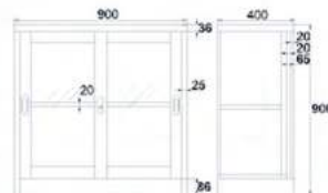
YD-B5 Sliding Glass Doors Cabinet W900 x D400 x H900 mm.
