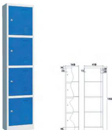
YD-CA4 Clothes Cabinet W380 x D450 x H1850 mm.
