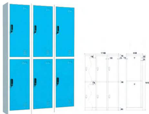
YD-CB6 Clothes Cabinet W1140 x D450 x H1850 mm.
