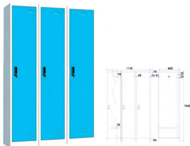
YD-CB3 Clothes Cabinet W1140 x D450 x H1850 mm.
