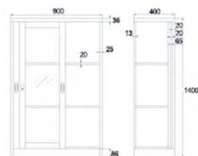
YD-B10 Sliding Glass Doors Cabinet W900 x D400 x H1400 mm.
