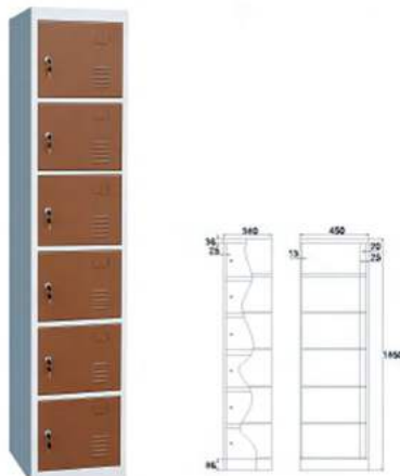
YD-CA6 Clothes Cabinet W380 x D450 x H1850 mm.
