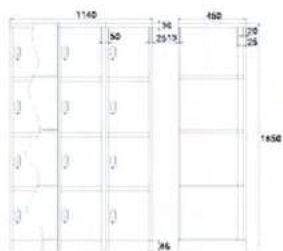
YD-CB12 Clothes Cabinet W1140 x D450 x H1850 mm.
