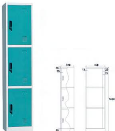
YD-CA3 Clothes Cabinet W380 x D450 x H1850 mm.
